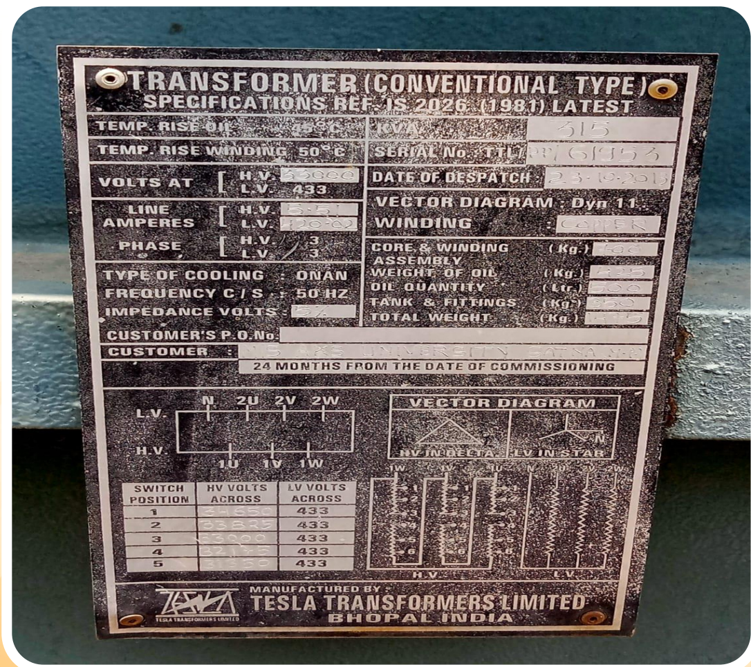
Photo 14: Transformer Specification
